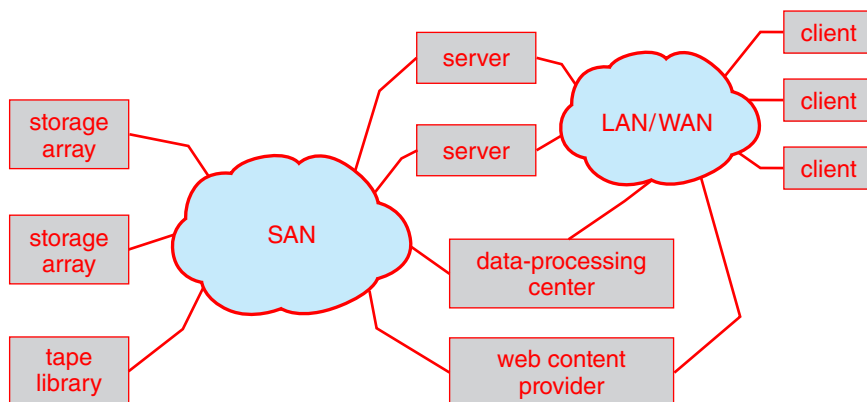
Figure 11.13 Storage-area network.
