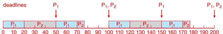
Figure 5.22 Rate-monotonic scheduling.
