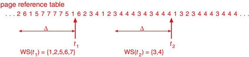
Figure 10.22 Working-set model.
