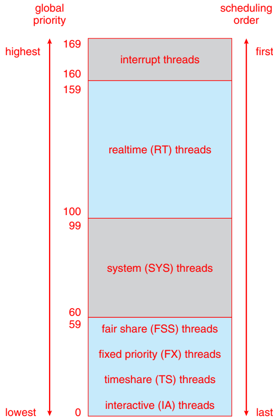
Figure 5.30 Solaris scheduling.
